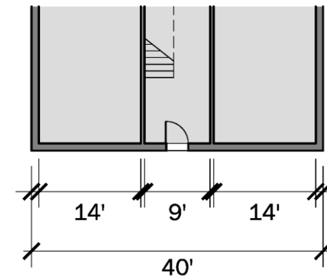
One example of a Partial floor plan view
